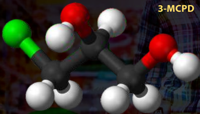
3-Chloropropane-1,2-diol
